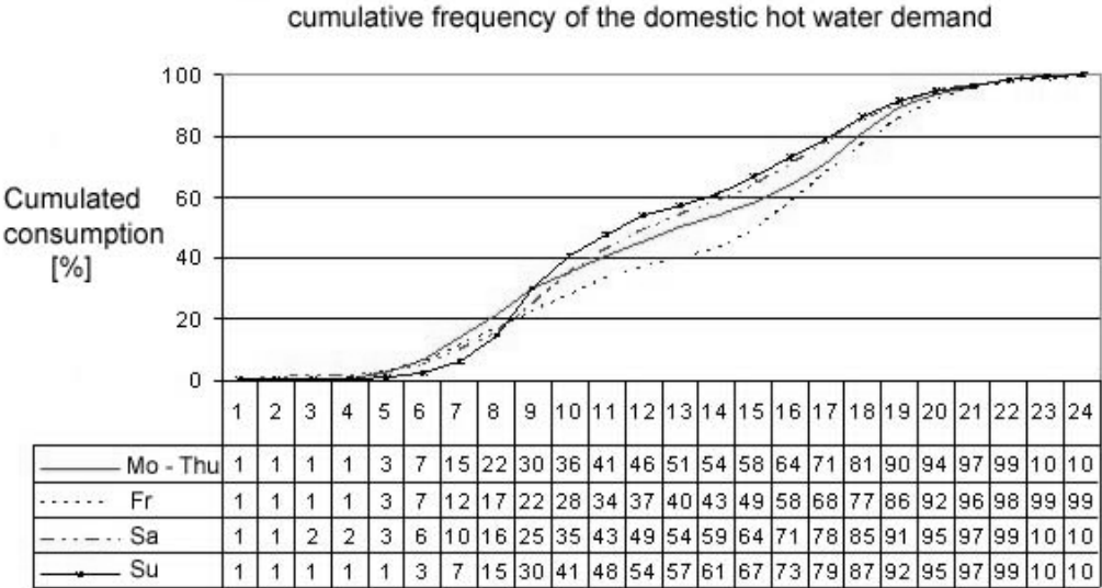
Fig. 14: tapping profile according to VSSH handbook
