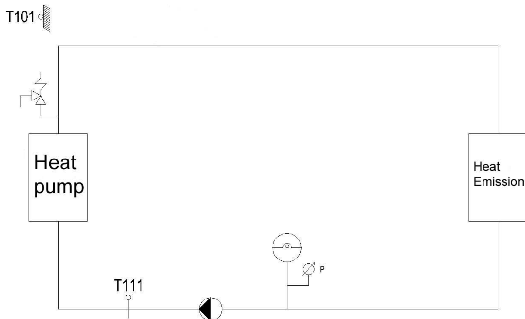
Fig. 23: hydraulic scheme of the system configuration P2 and P5
