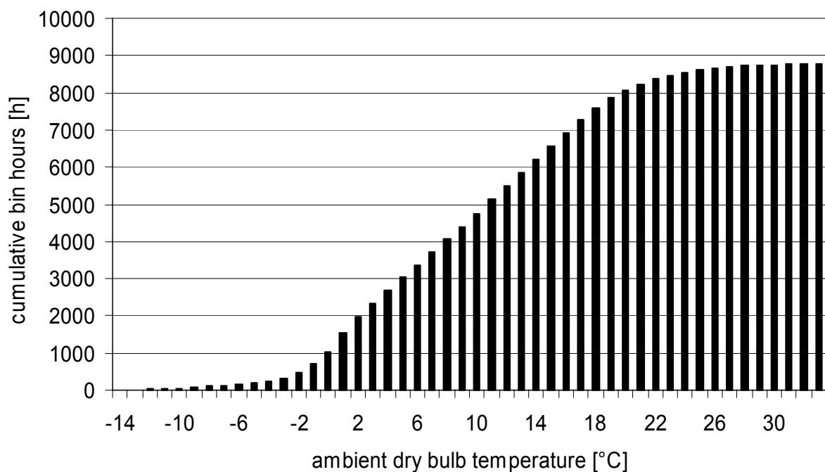
Fig. 9: cumulative annual frequency of the ambient dry bulb temperature
