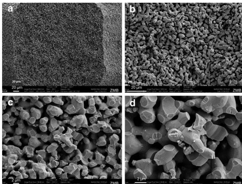
FIG. 2. SEM of a broken TCP rod. (a–d) Shows the final scaffold after sintering. Scales are provided in the panels. TCP particles and micropores appear 2–4 \mu\text{m} in diameter. SEM, scanning electron microscopy.
