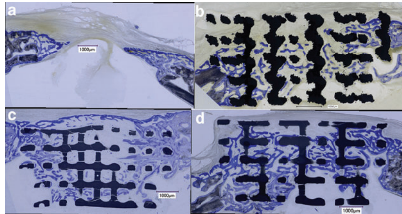
FIG. 3. Histological sections from the middle of the noncritical-size defect. (a–d) For all scaffolds and the untreated control, a histological section from 4 weeks postoperatively is shown. (a) Empty control defect; (b) titanium scaffold; (c) TCP scaffold with 10 \mu g BMP-2; (d) TCP scaffold. Scale bars indicate 1 mm. Original magnifications were 100 fold. Bone appears as grayish purple to purple, titanium as dark black, and TCP as grayish black. BMP, bone morphogenetic protein. Color images available online at www.liebertpub.com/tea
