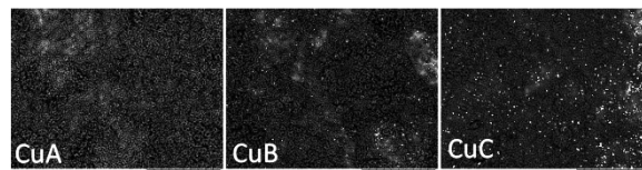
Fig. 1: Scanning electron microscope images of titanium discs with Cu deposits (white spots); CuA: 1.6 \pm 0.5 \mu g/disc; CuB: 18.7 \pm 3.1 \mu g/disc, CuC: 49.7 \pm 5.5 \mu g/disc (x600; TM3000 Hitachi; 15 kV; backscattered electrons).
